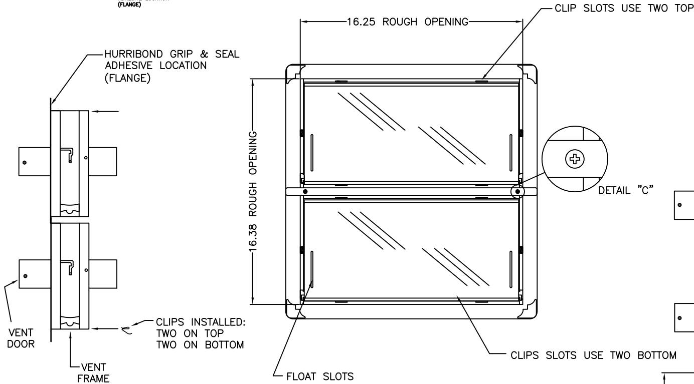
FIGURE 2 SIDE VIEW
