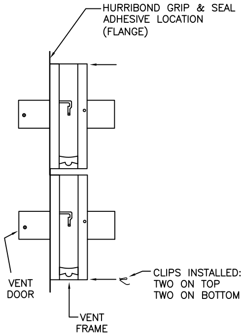
FIGURE 2 SIDE VIEW
